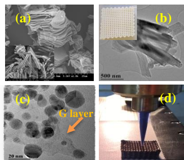
Fig. 1: Electron microscopy images of (a) MXene (inset Mxene rods), (b) h-BN and inset corresponding 3D printed compound, (c) Ag-graphene, (d) 3D printed graphene nanocomposites.
