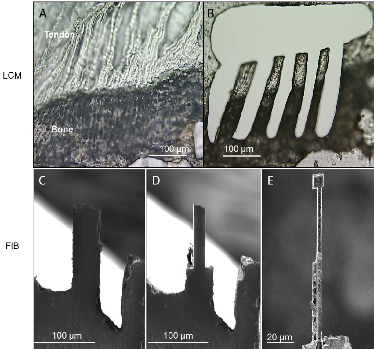
Figure 1: Murine tendon-to-bone attachment sites were cut and milled to beams measuring approximately 60 \mu m long and 4.5 by 4.5 \mu in diameter. (A) Dissected supraspinatus-to-humeral head complexes were fresh frozen and sectioned into 20-30 \mu m thick slices. (B) LCM was used to cut large beams, \sim 250 \mu m by 50 \mu m by 20-30 \mu m, in the fibrocartilaginous region of the attachment where there is a gradient in mineralization. (C-E) The LCM cut beams were further milled down to the final small beams via cryo-FIB.
