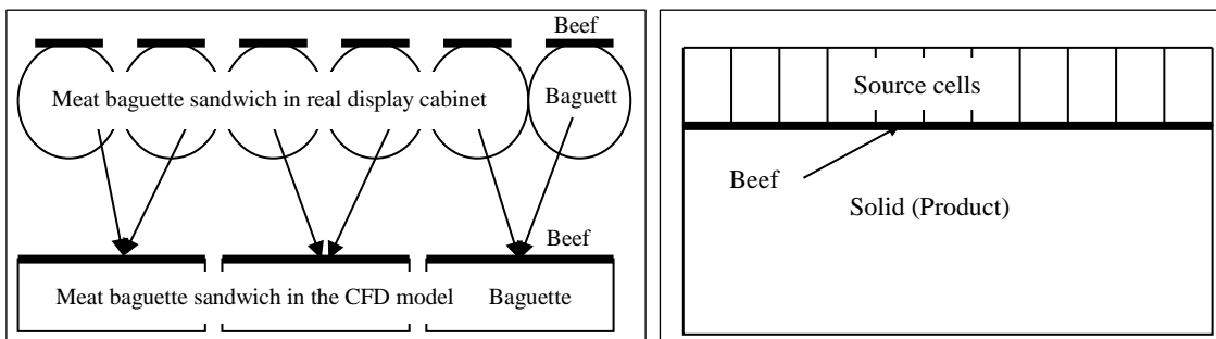
Fig. 2. (a) Representation of the sandwiches in the 2D CFD model of the serve-over display cabinet (b) Cross-Section of the Beef Baguette Sandwich with Water Vapour Source Cells
